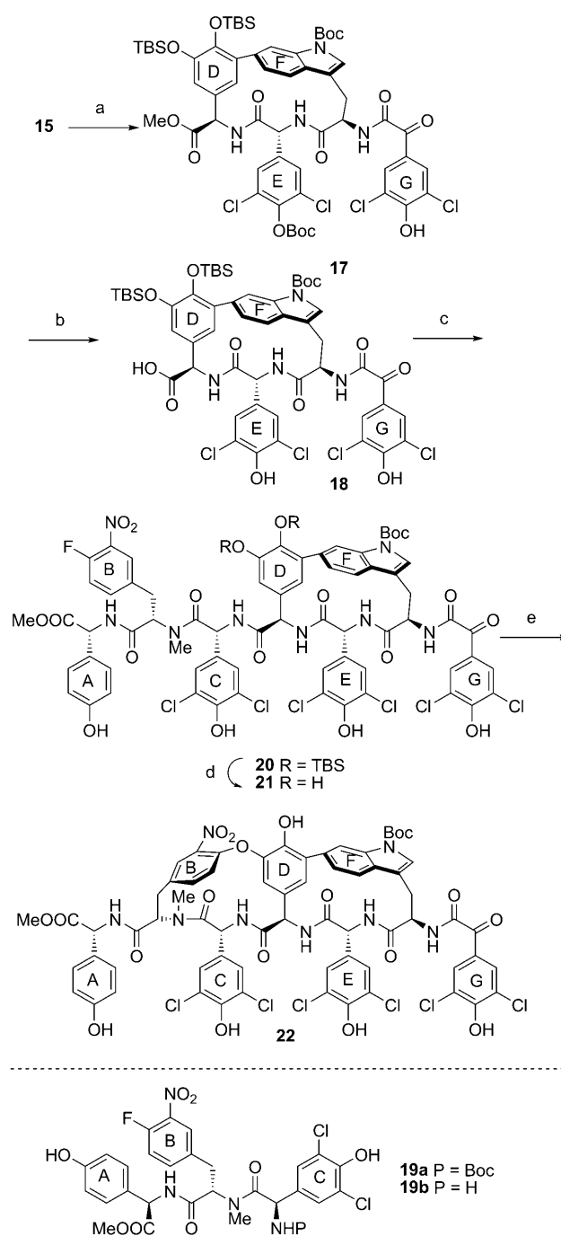
Scheme 2. a) \text{Boc}_2\text{O} (10 equiv), DMAP (0.4 equiv), MeCN/ \text{H}_2\text{O} (v/v = 1000:1, c = 0.003 M), RT, overnight; b) \text{Me}_3\text{SnOH} , \text{ClCH}_2\text{CH}_2\text{Cl} , 80 °C, 3 days, 48 % yield over 2 steps; c) tripeptide 19b , HATU (1.5 equiv), THF, 60 % yield; d) KF (20 equiv), conc. aqueous HBr in DMF (0.03 M, 3 equiv), RT, 2 h; e) \text{K}_2\text{CO}_3 , DMSO, 4 Å M.S., 30 °C, 20 h, 62 % yield over 2 steps.
