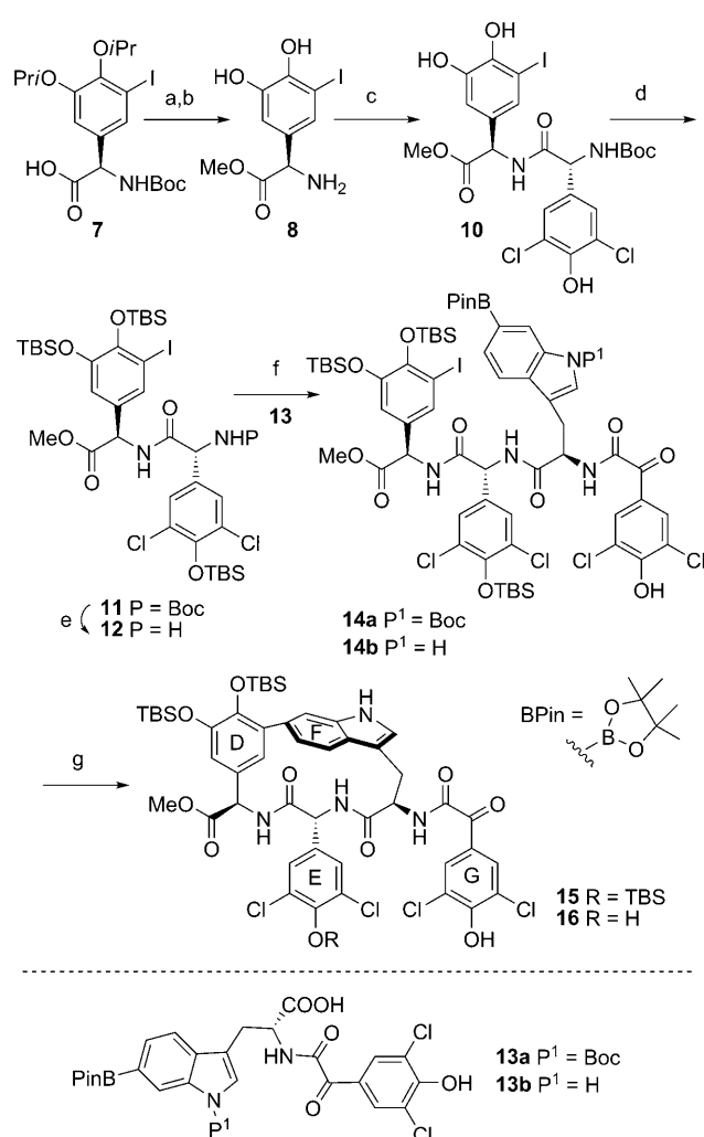
Scheme 1. a) SOCl_2 , MeOH; b) BCl_3 , CH_2Cl_2 ; c) D- N -Boc-3,5-dichloro-4-hydroxyphenylglycine ( 9 ), DEPBT, NaHCO_3 , THF; d) TBSCl (9 equiv), imidazole (18 equiv), DMF, 40 °C, 65 % yield over 4 steps; e) 12 M HCl in MeCN (v/v = 0.07); f) HATU, 2,5-lutidine, CH_2Cl_2 /THF, 80 % yield; g) [PdCl_2(dppf)] \cdot CH_2Cl_2 (1 equiv), K_2CO_3 (10 equiv), dioxane/ H_2O (15:1), 90 °C, 66 % yield. HATU = O-(7-azabenzotriazol-1-yl)- N,N,N',N' -tetramethyluronium hexafluorophosphate; TBS = tert -butyldimethylsilyl; DMF = N,N -dimethylformamide; DEPBT = 3-(diethoxyphosphoryloxy)-1,2,3-benzotriazin-4(3 H )-one; dppf = 1,1'-bis(diphenylphosphino)ferrocene; Boc = tert -butoxycarbonyl.
