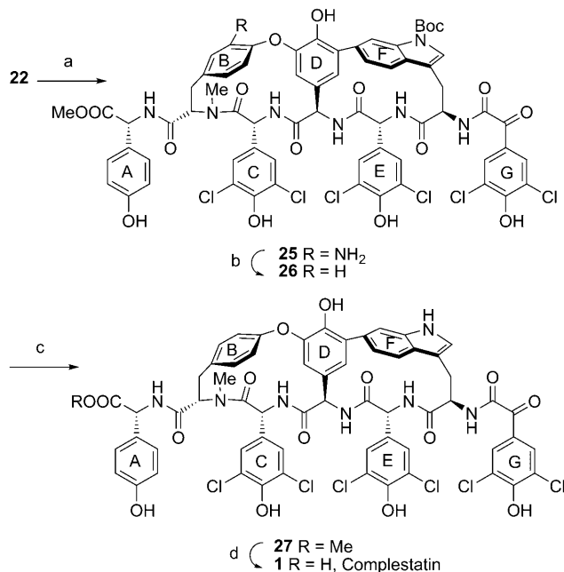
Scheme 4. a) SnCl_2 , MeOH, 60 °C, 78% yield; b) tBuONO , H_3PO_2 , THF, 0 °C, 82% yield; c) trifluoroethanol, microwave irradiation, 100 °C; d) LiOH, THF/ H_2O , 0 °C, 83% yield over 2 steps.
