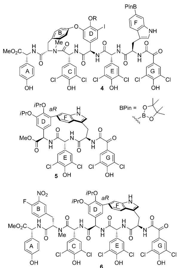
Scheme 1. a) SOCl_2 , MeOH; b) BCl_3 , CH_2Cl_2 ; c) D- N -Boc-3,5-dichloro-4-hydroxyphenylglycine ( 9 ), DEPBT, NaHCO_3 , THF; d) TBSCl (9 equiv), imidazole (18 equiv), DMF, 40 °C, 65 % yield over 4 steps; e) 12 M HCl in MeCN (v/v = 0.07); f) HATU, 2,5-lutidine, CH_2Cl_2 /THF, 80 % yield; g) [PdCl_2(dppf)] \cdot CH_2Cl_2 (1 equiv), K_2CO_3 (10 equiv), dioxane/ H_2O (15:1), 90 °C, 66 % yield. HATU = O-(7-azabenzotriazol-1-yl)- N,N,N',N' -tetramethyluronium hexafluorophosphate; TBS = tert -butyldimethylsilyl; DMF = N,N -dimethylformamide; DEPBT = 3-(diethoxyphosphoryloxy)-1,2,3-benzotriazin-4(3 H )-one; dppf = 1,1'-bis(diphenylphosphino)ferrocene; Boc = tert -butoxycarbonyl.
